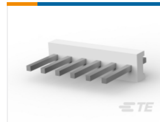
TE Part # 640383-6 06P MTA156 HDR ASSY STR SQ SN
